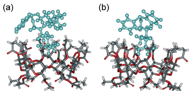
Figure 5. Side view of the computer-generated structure of the (a) Per-Ac- \beta -CD/2 and (b) Per-Ac- \beta -CD/3 inclusion complexes.
