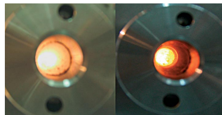
Figure 6. View of the autoclave window for the [\text{Rh}(\text{acac})(\text{CO})_2]/1/\text{Per-Ac-}\beta\text{-CD} system at 80 °C and at (a) 200 atm and (b) 250 atm (solubilised).
