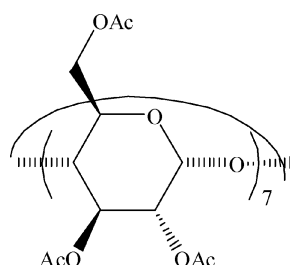
Figure 2. Peracetylated cyclodextrin (Per-Ac- \beta -CD).
