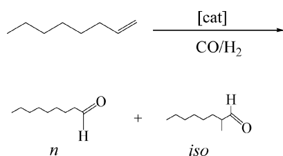
Scheme 1. Hydroformylation of 1-octene.
