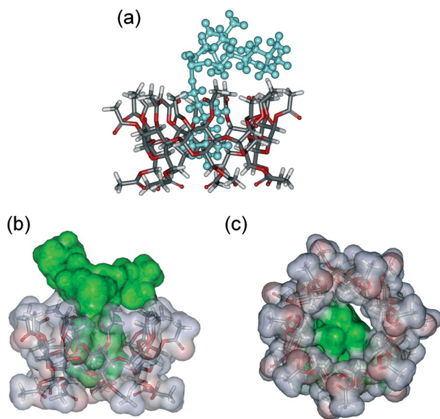
Figure 4. (a) Side view of the computer-generated structure of the Per-Ac- \beta -CD/1 inclusion complex. (b) Side view and (c) bottom view of the van der Waals surfaces of the Per-Ac- \beta -CD/1 inclusion complex.
