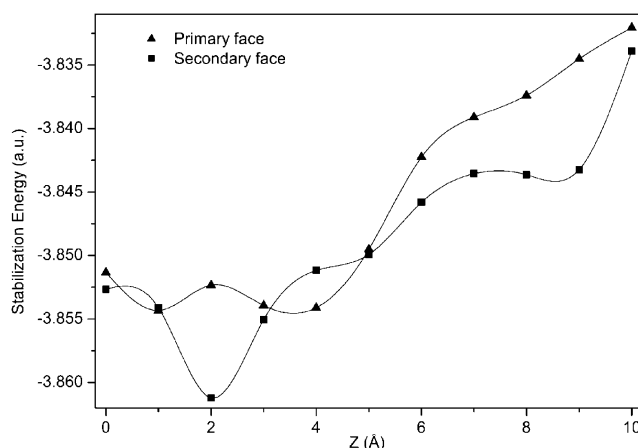
Figure 3. Graphic diagram for the inclusion process of the phosphite 1 with Per-Ac- \beta -CD through the primary ( \blacktriangle ) and secondary ( \blacksquare ) faces.
