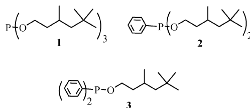
Figure 1. P-donor ligands containing a branched alkylic chain used in the hydroformylation of 1-octene in scCO 2 : phosphite ligand ( 1 ), phosphonite ligand ( 2 ) and phosphinite ligand ( 3 ).
